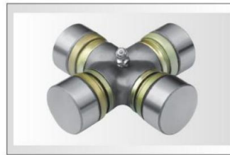
GUM-72 MITSUBISHI OEM:13518-2200 ★ Universal joint Φ36X104
